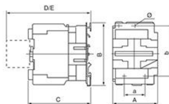
CJX2-D40~95
