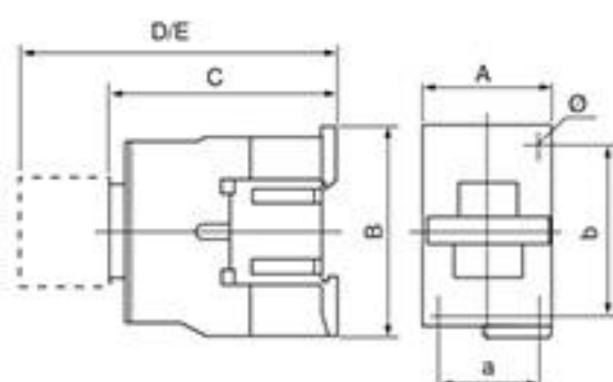
CJX2-D09~32
